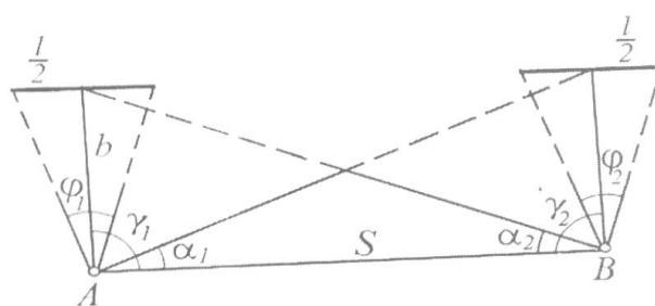
Рис.14 S_{AB} = l/2 \operatorname{ctg} \varphi_1 / 2 \sin(\gamma_1 + \alpha_2) \operatorname{cosec} \alpha_2 S_{AB} = l/2 \operatorname{ctg} \varphi_2 / 2 \sin(\gamma_2 + \alpha_1) \operatorname{cosec} \alpha_1
